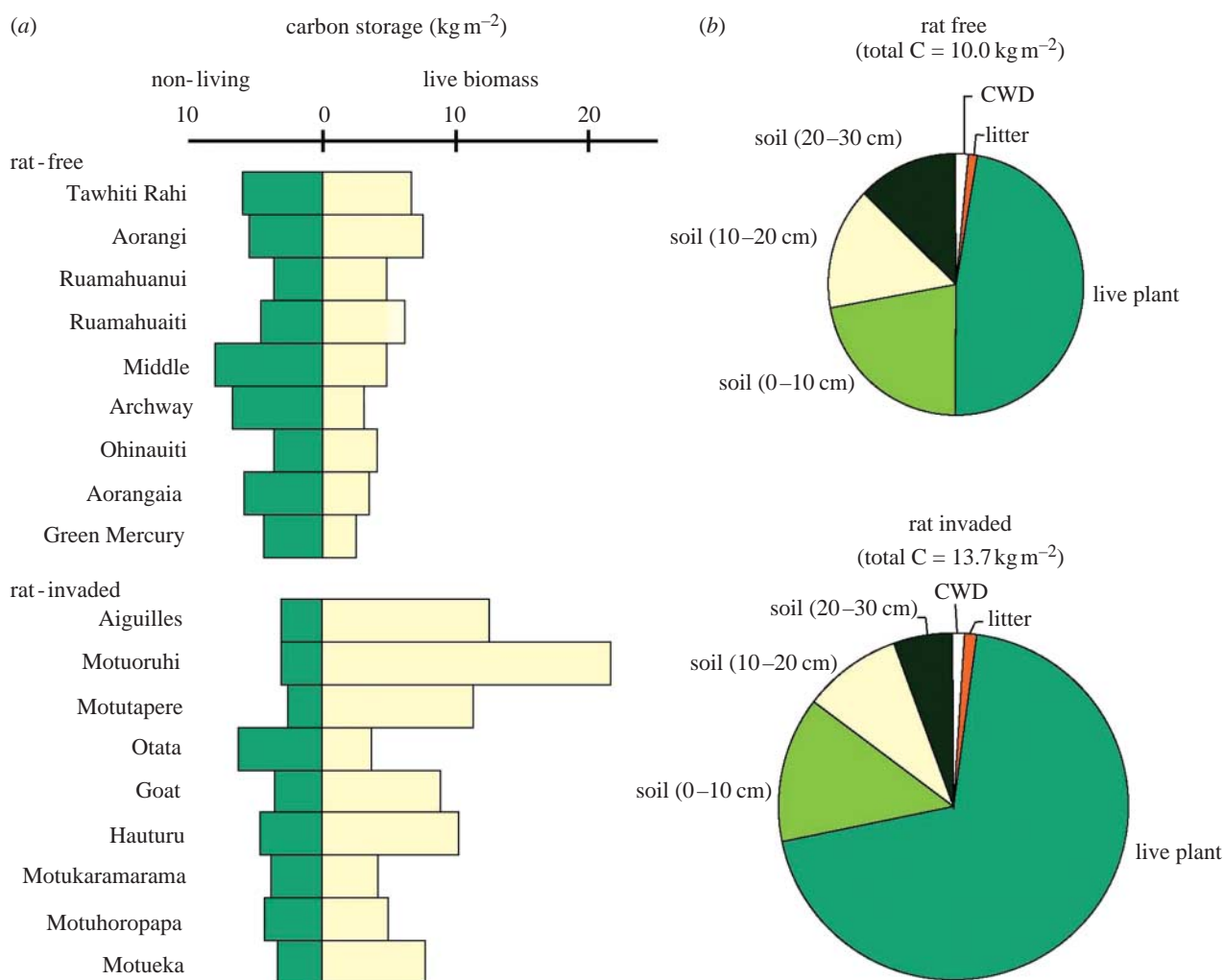
Figure 1. (a) Carbon storage in live plant biomass and in non-living pools (soil, litter and CWD) on nine rat-free (seabird-dominated) and nine rat-invaded islands. For both categories, islands are arranged in decreasing order of size. (b) Proportions of total ecosystem C stored in different pools for rat-free and rat-invaded islands. Data analyses and significance tests are presented in table 1.
